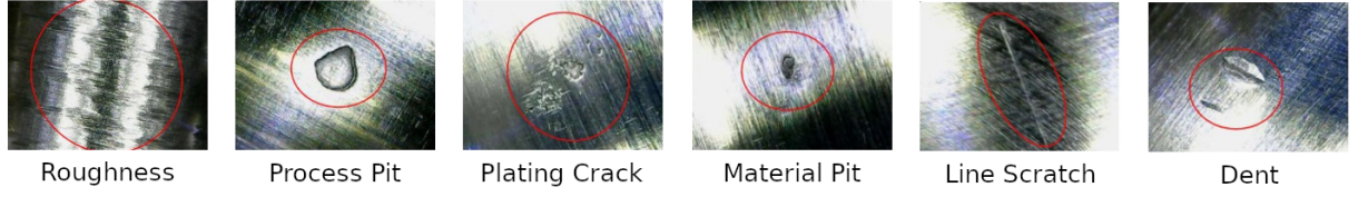
Figure 3.2: Defects on steel rods from Agriauto dataset
